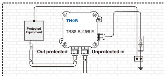
IP68 WATERPROOF PROTECTION FOR USE IN OUTDOOR
