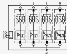
Basic circuit diagram
