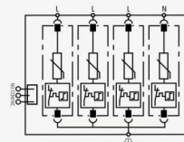
Basic circuit diagram
